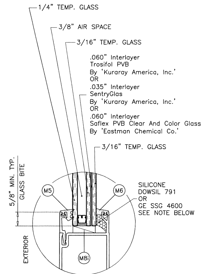
GLASS TYPE 'A3i'
